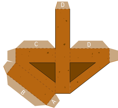
Hitch Posts
